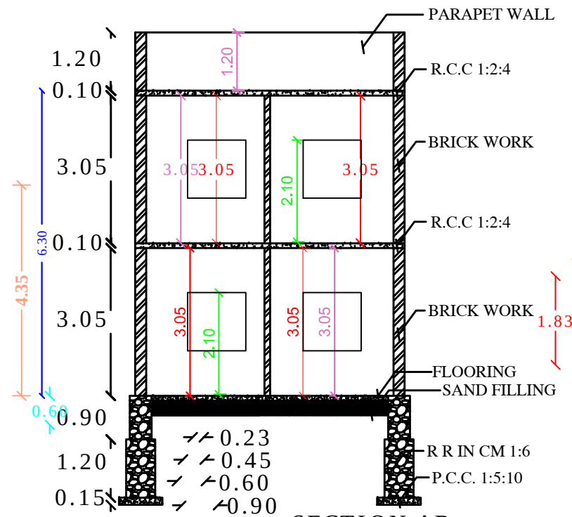
SECTION AB
