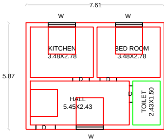
PROPOSED FF PLAN
