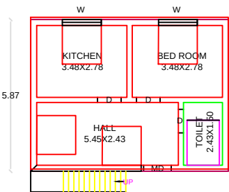
PROPOSED GF PLAN
