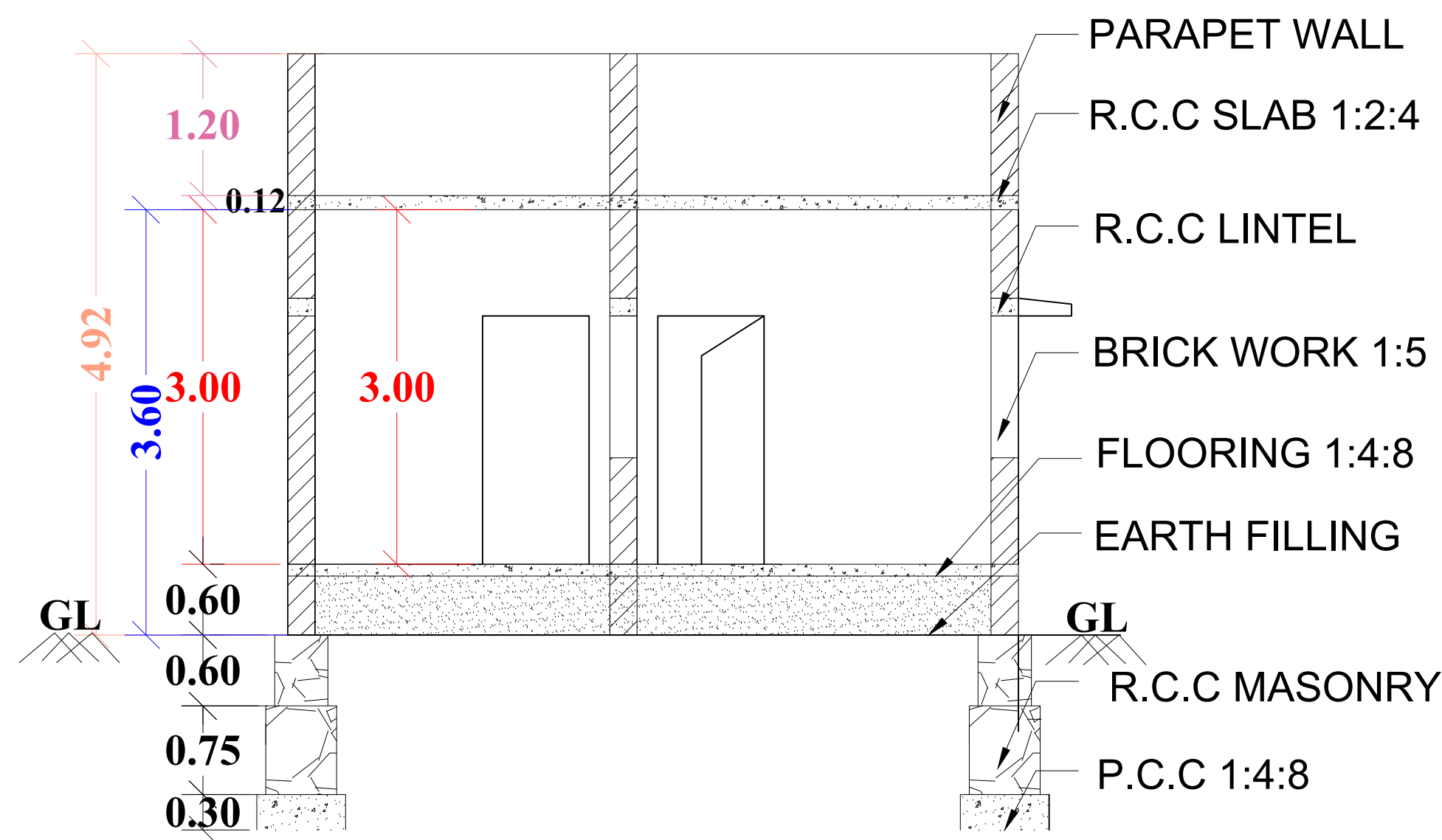
"SECTION "AB"
