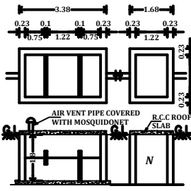
PLAN/SECTION OF SEPTIC TANK 'U' TRAP PROVIDED
