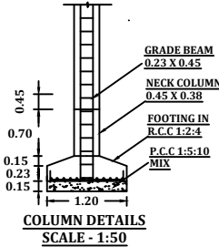
COLUMN DETAILS SCALE - 1:50
