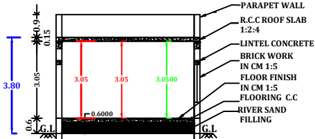
SECTION ON AA1
