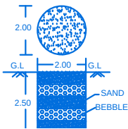
SECTION ON 'AA'
