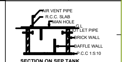
SECTION ON SEP.TANK
