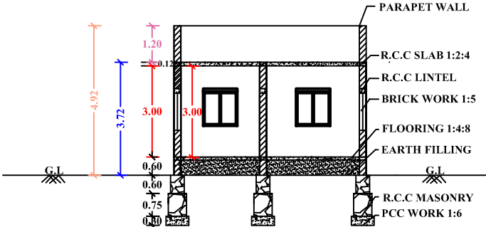
"SECTION "AB"
