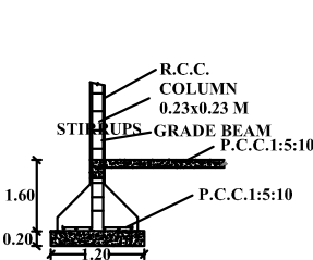
COLUMN DETAIL
