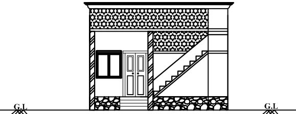
"SECTION "AB"
