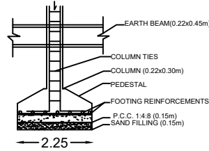
FOUNDATION DETAILS
