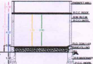
CROSS SECTION
