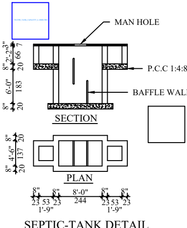
SEPTIC-TANK DETAIL
