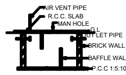
SECTION ON SEP. TANK
