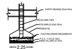
FOUNDATION DETAILS
