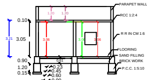
SECTION AB
