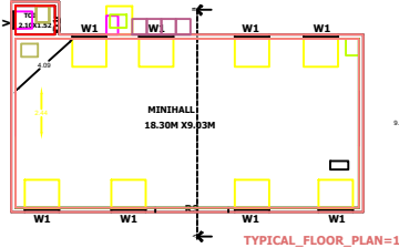
TYPICAL_FLOOR_PLAN=1
