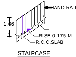
STAIRCASE
