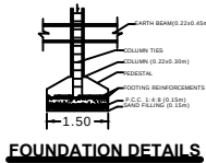
FOUNDATION DETAILS
