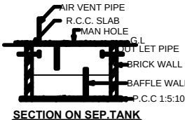
SECTION ON SEP. TANK
