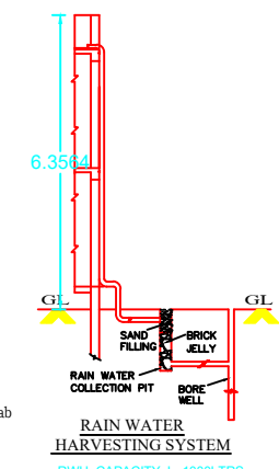
RAIN WATER HARVESTING SYSTEM RWH_CAPACITY_L=1000LTRS
