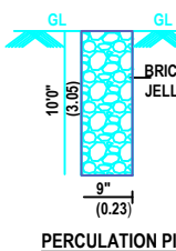
PERCOLATION PIT
