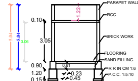
SECTION AB
