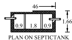
PLAN ON SEPTICTANK
