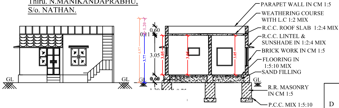
SECTION OF "AB"
