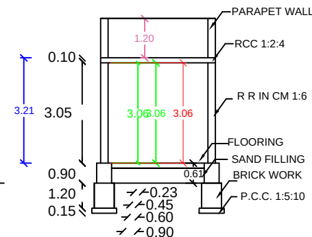
SECTION AB
