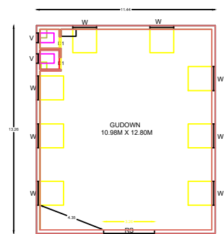
TYPICAL_FLOOR_PLAN=1 GROUND FLOOR PLAN
