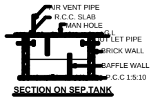
SECTION ON SEP.TANK
