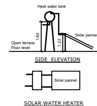
SOLAR WATER HEATER
