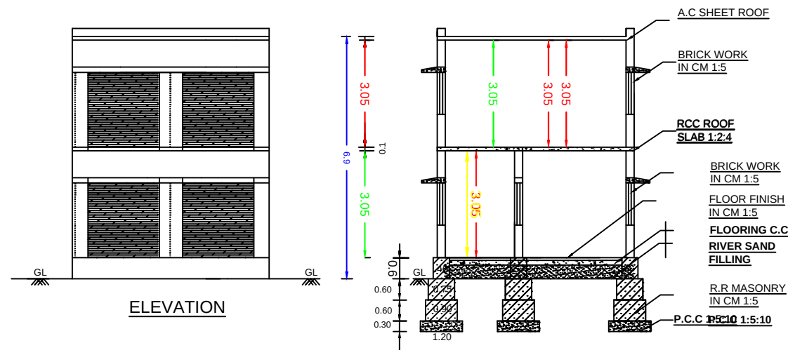
SECTION ON AA1
