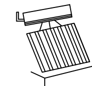
SOLAR SYSTEM
