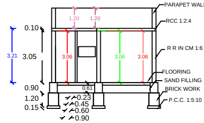
SECTION AB
