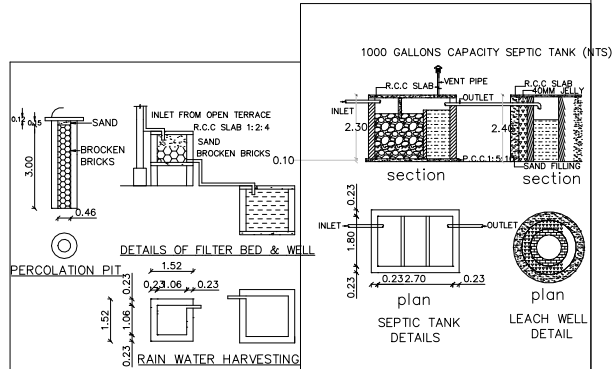
RAIN WATER COLLECTING TANK
