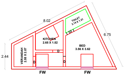
PLAN - FIRST FLOOR (PROPOSED)
