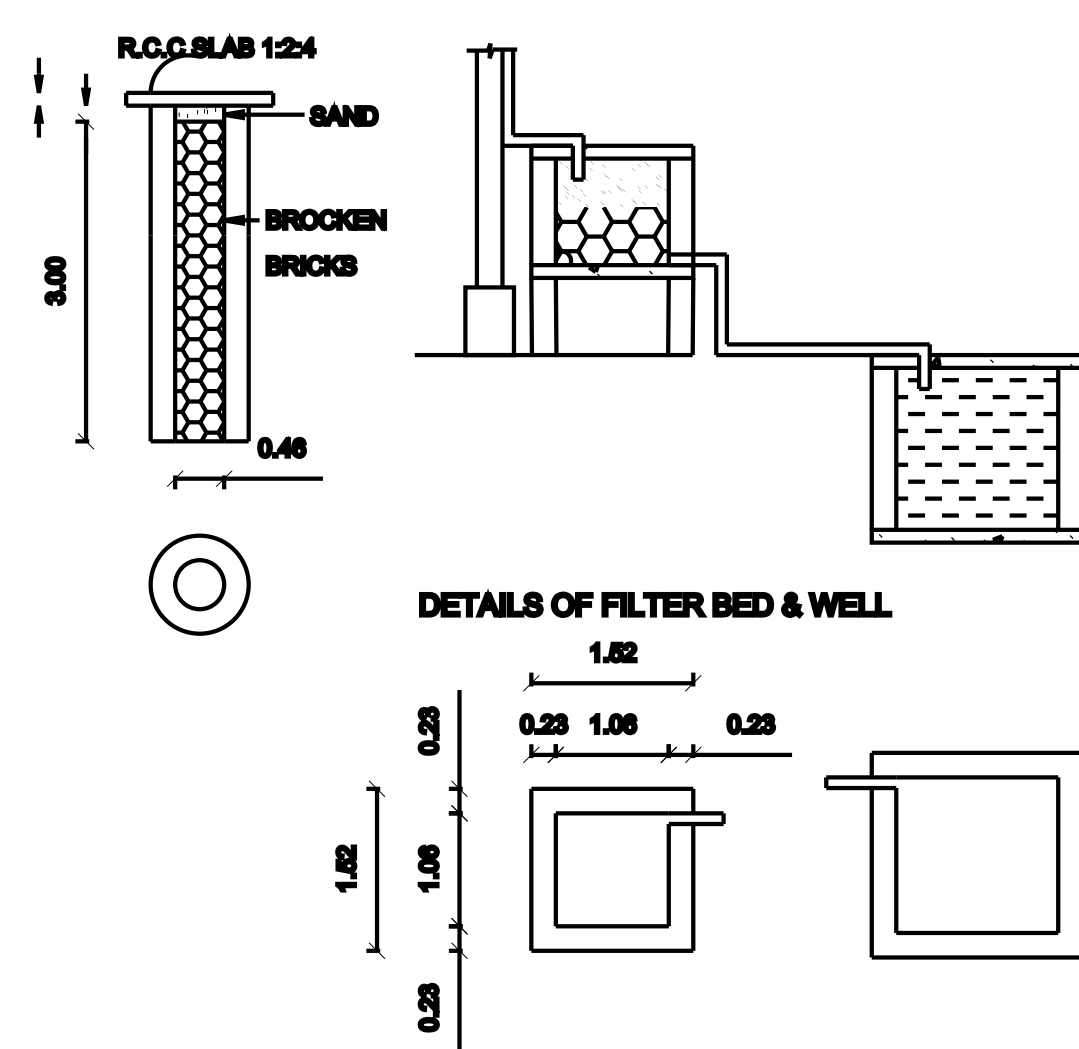
SEPTIC TANK DETAILS
