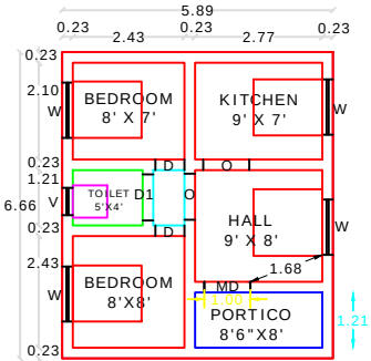
GROUND FLOOR RESIDENTIAL PLAN
