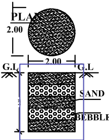
RAIN WATER HARVESTING
