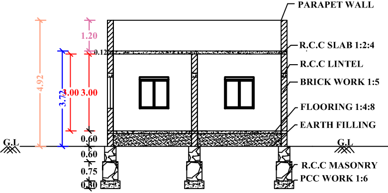
"SECTION "AB"
