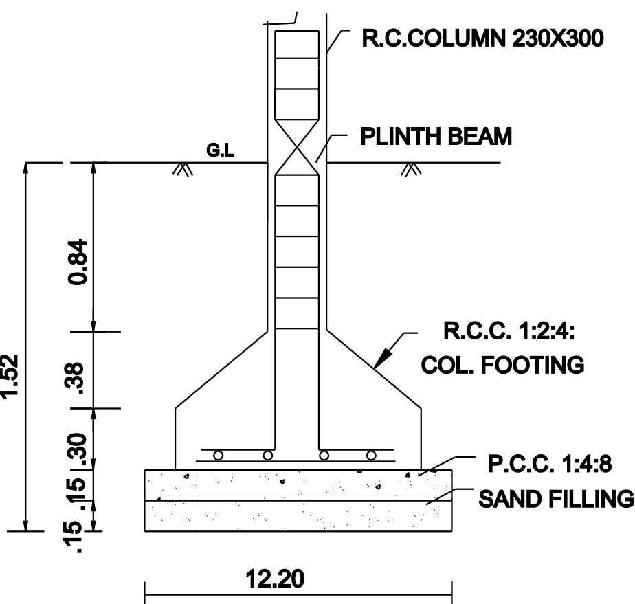
FOUNDATION DETAIL
