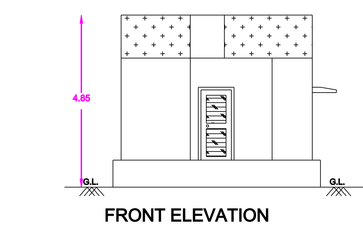
FRONT ELEVATION
