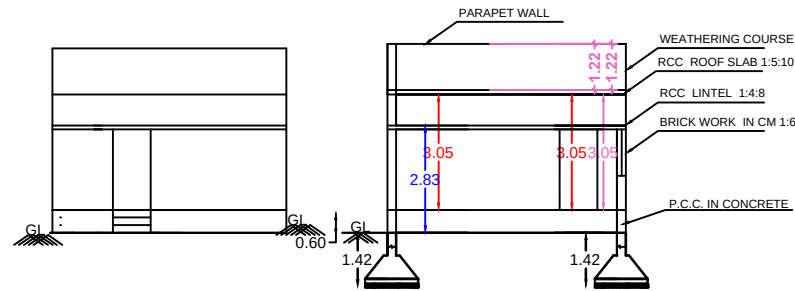
ELEVATION SECTION ON AA
