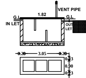
SEPTICTANK DETAILS
