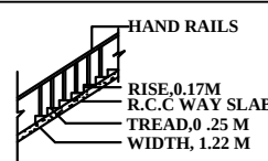
SECTION ON STAIR
