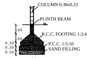
COLUMN DETAILS
