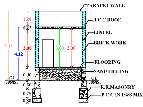
"SECTION "AB"
