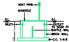
SECTION OF SEPTIC TANK
