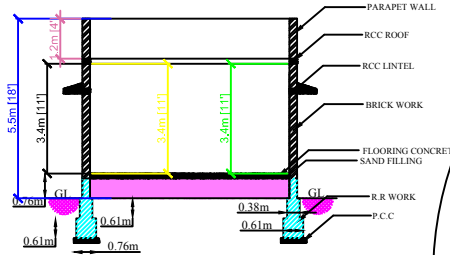
SECTION AB
