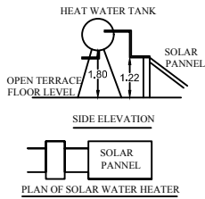
PLAN OF SOLAR WATER HEATER
