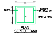
PLAN SEPTIC TANK
