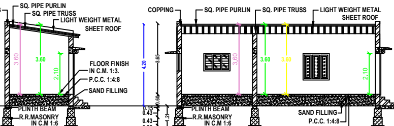
SECTION ON 'BB'
