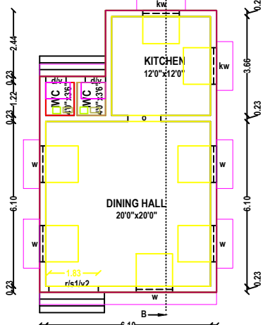
PLAN - RESTAURENT ( LIGHT WEIGHT METAL SHEET ROOF )
