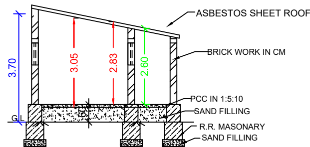
SECTION "AB"
