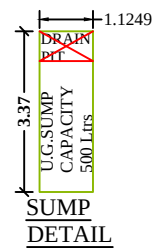
SUMP DETAIL
