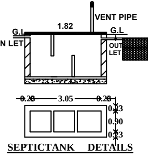
SEPTICTANK DETAILS
