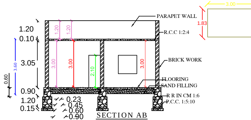
SECTION AB PEER MOHAMMED LAND 20'0" (6.10)
