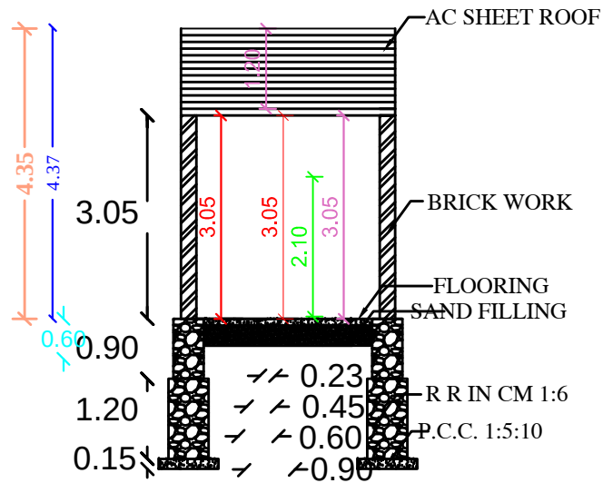
SECTION AB MARIAPPAN & SANTHANAKUMAR LAND
