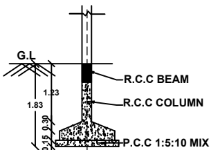
SECTION OF FOOTING
