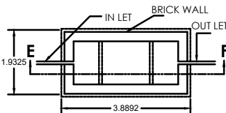
PLAN PLAN OF SEPTIC TANK
