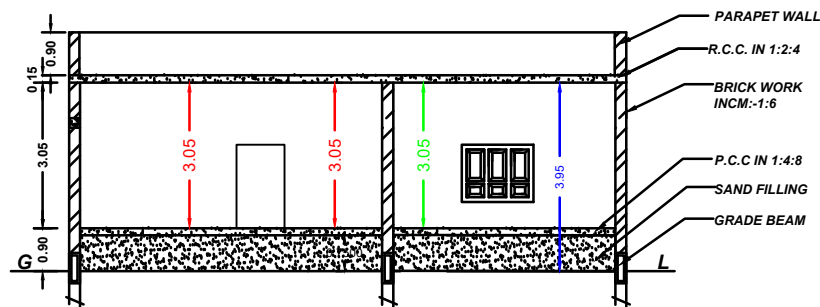
SECTION "AB"
