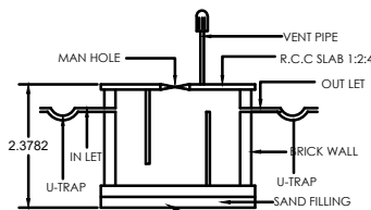
SECTION E.F. SEPTIC TANK DETAIL
