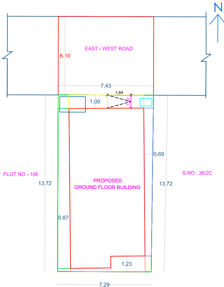
LOCATION PLAN
