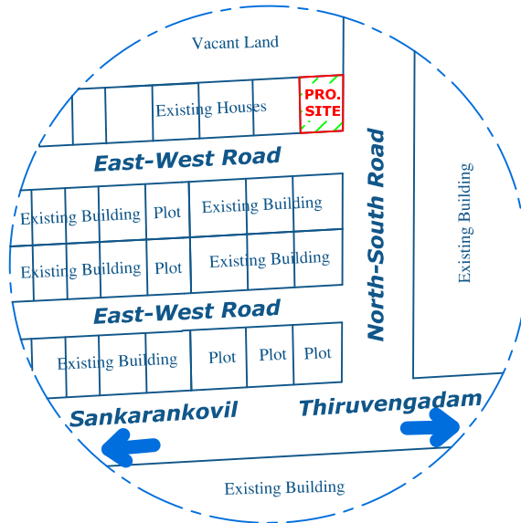
LOCATION PLAN
