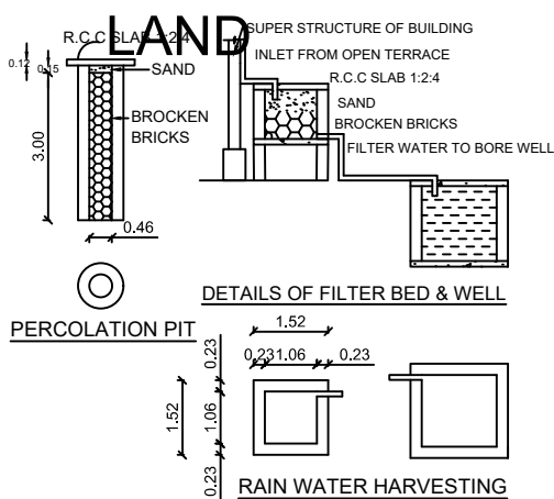
DETAILS OF FILTER BED & WELL
