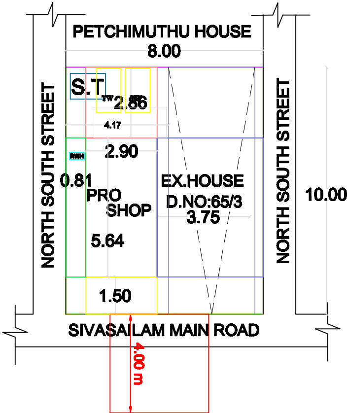
SITE PLAN
