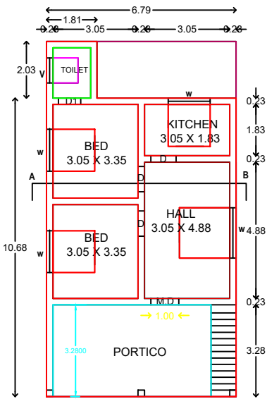
G.FLOOR PLAN
