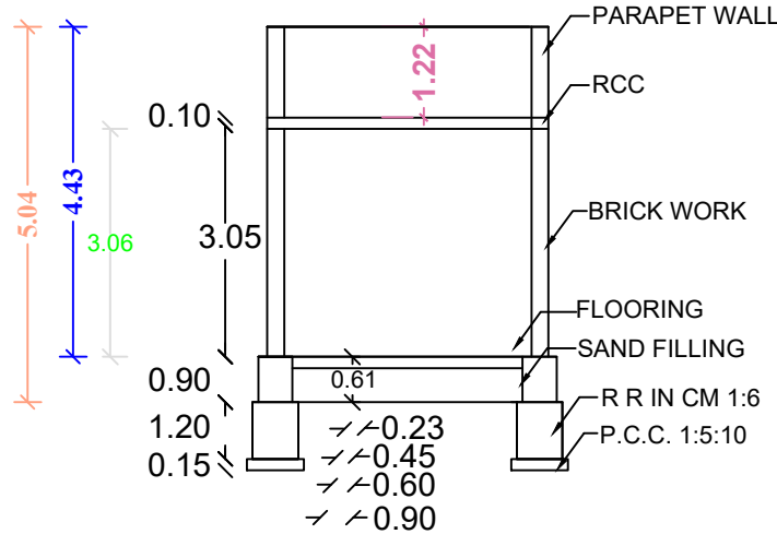
SECTION AB
