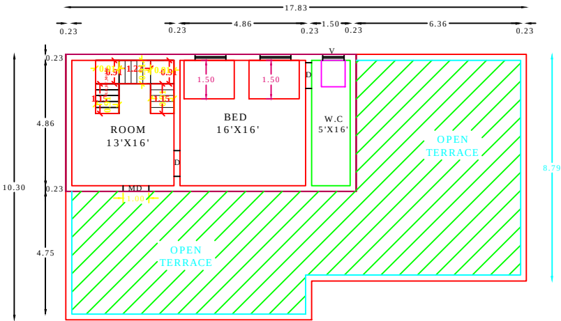
PRO FIRST FLOOR RESIDENTIAL PLAN
