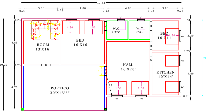
PRO GROUND FLOOR RESIDENTIAL PLAN
