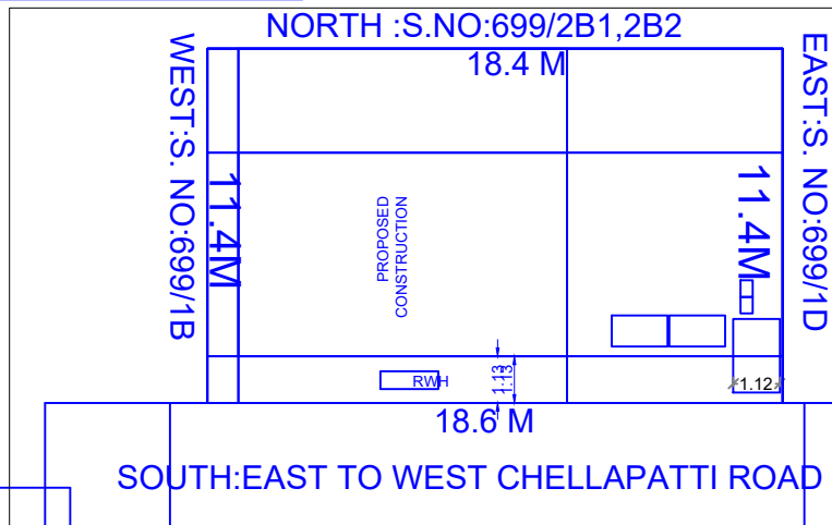
LOCATION PLAN SCALE 1:150
