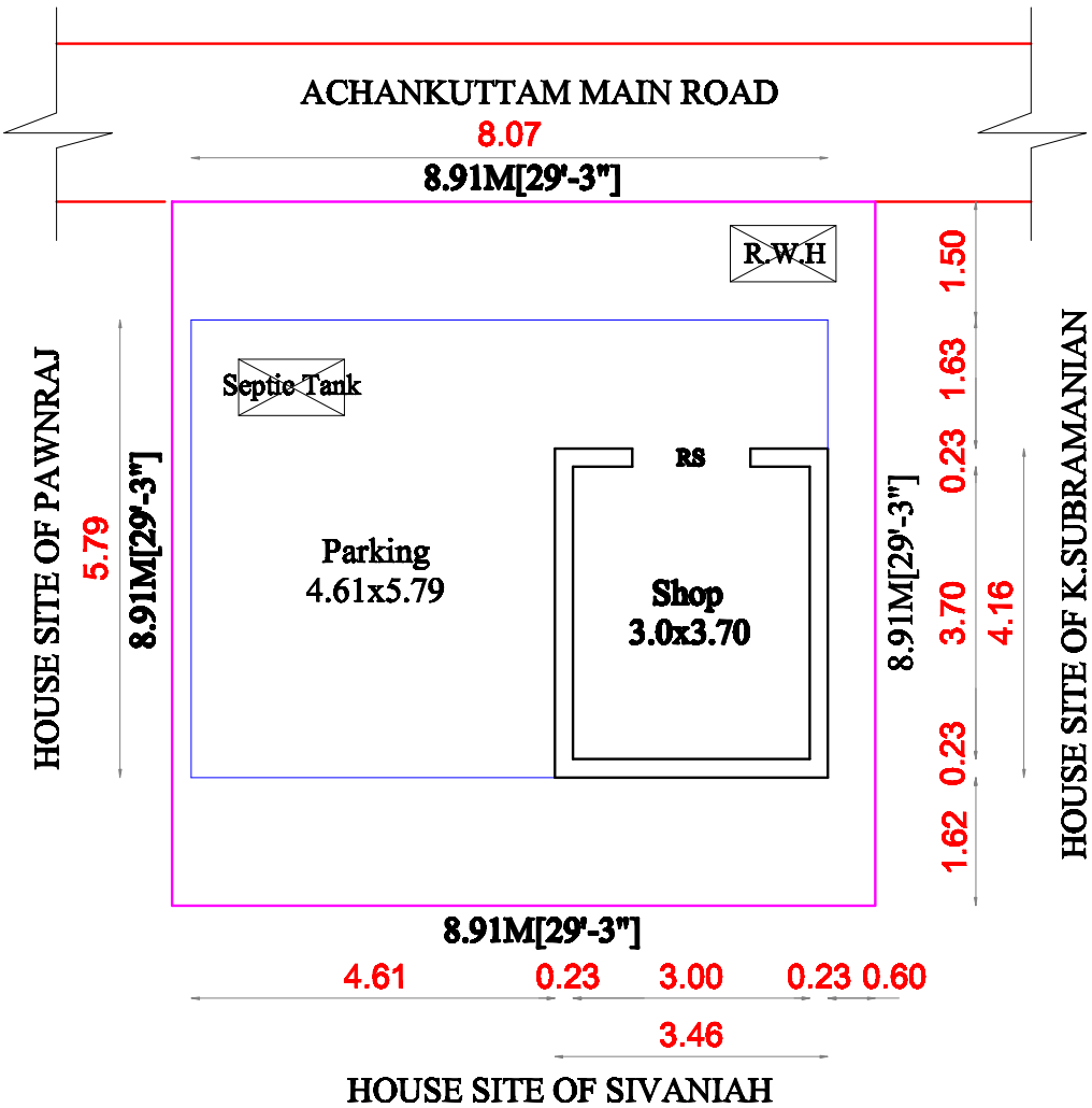
SITE CUM GROUND FLOOR PLAN
