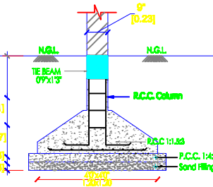
FOUNDATION DETAIL
