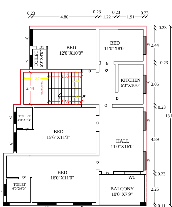
EXG.GROUND FLOOR PLAN
