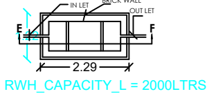
PLAN PLAN OF SEPTIC TANK
