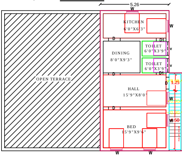
PRO.FIRST FLOOR PLAN
