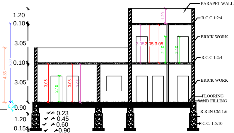
SECTION AB
