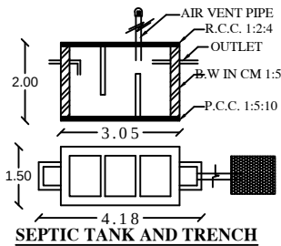
SEPTIC TANK AND TRENCH
